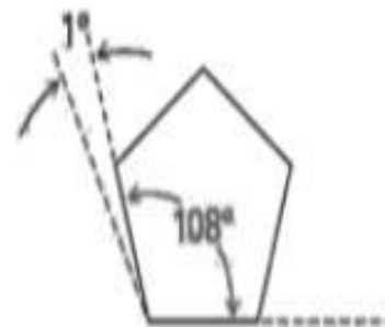
Cyclopentane
