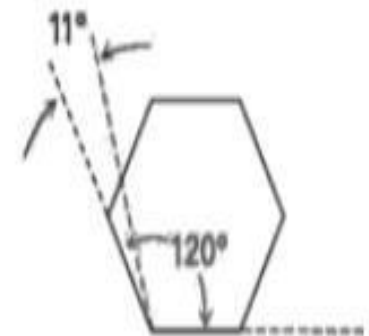
Cyclohexane
