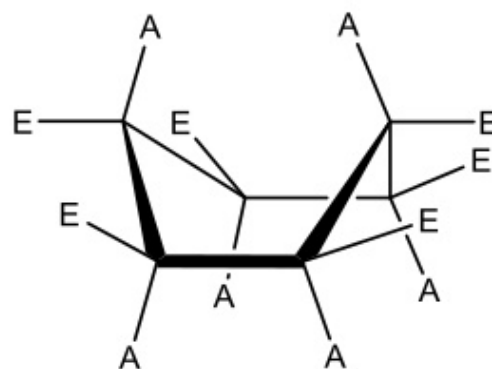
Boat conformation of cyclohexane
