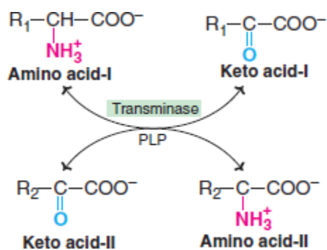
Figure2. Transamination reaction
